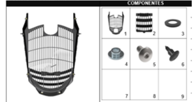
FIGURA 24: PARRILLA FRONTAL
