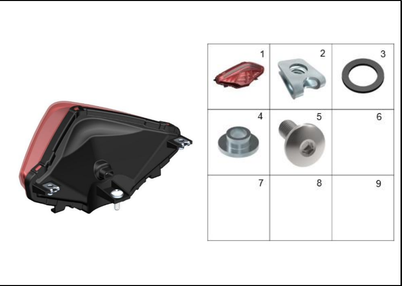
FIGURA 36: STOP
