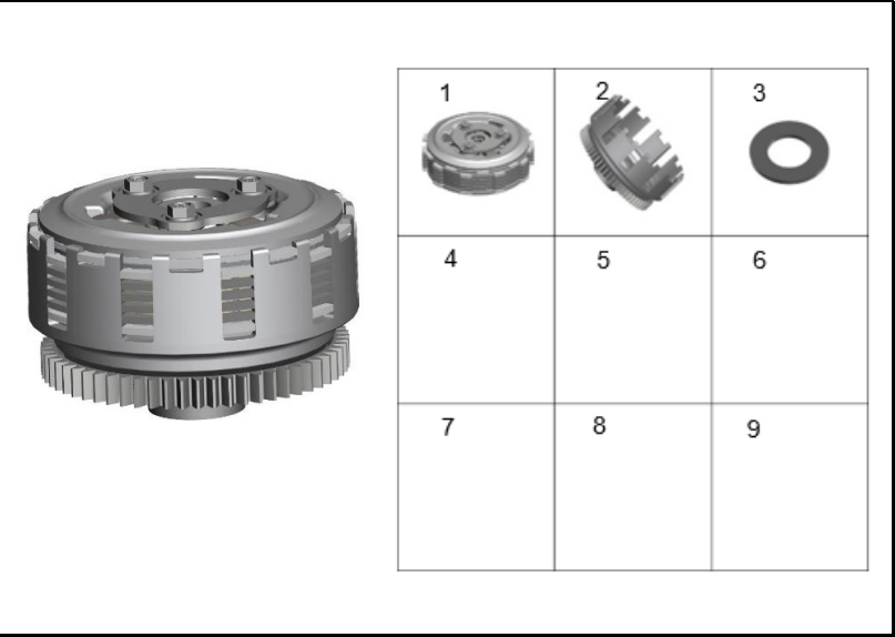
FIGURA 114: CLUTCH 2
