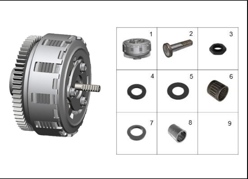
FIGURA 113: CLUTCH
