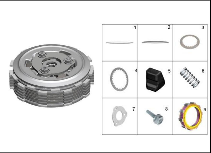
FIGURA 115: CLUTCH 3
