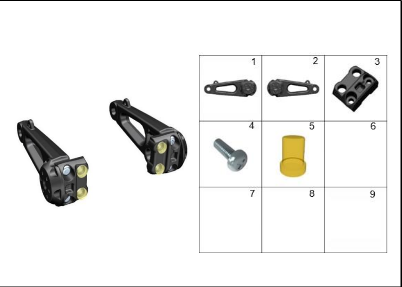
FIGURA 5: BALANCIN VISOR 2
