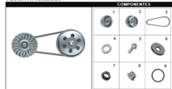
FIGURA 111: TRANSMISION
