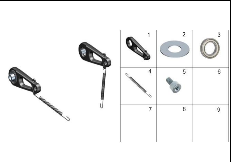
FIGURA 4: BALANCIN VISOR
