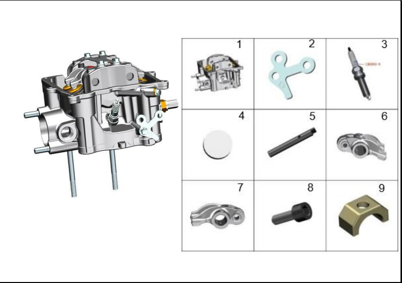
FIGURA 105: CULATA - BALANCINES
