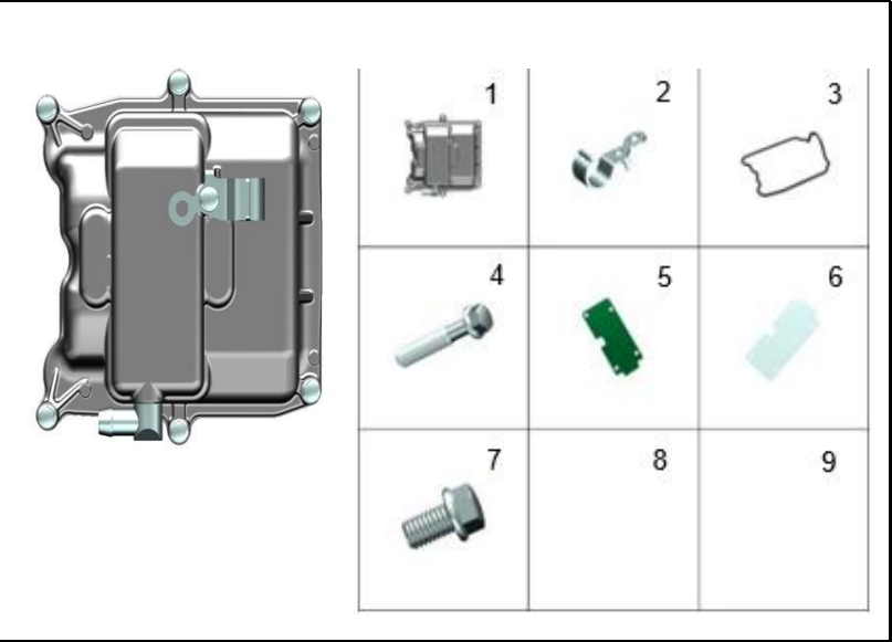
FIGURA 104: TAPA CULATA
