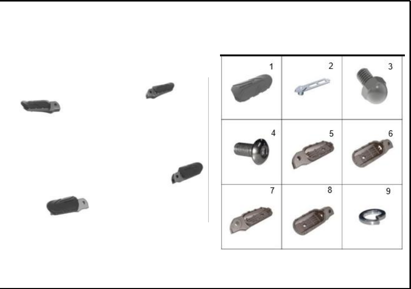
FIGURA 83: BASE REPOSAPIE
