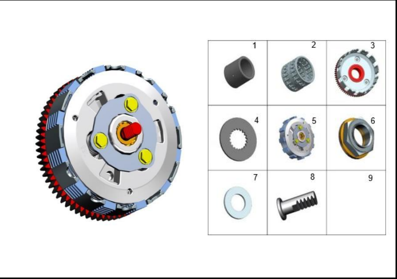
FIGURA 124: CLUTCH
