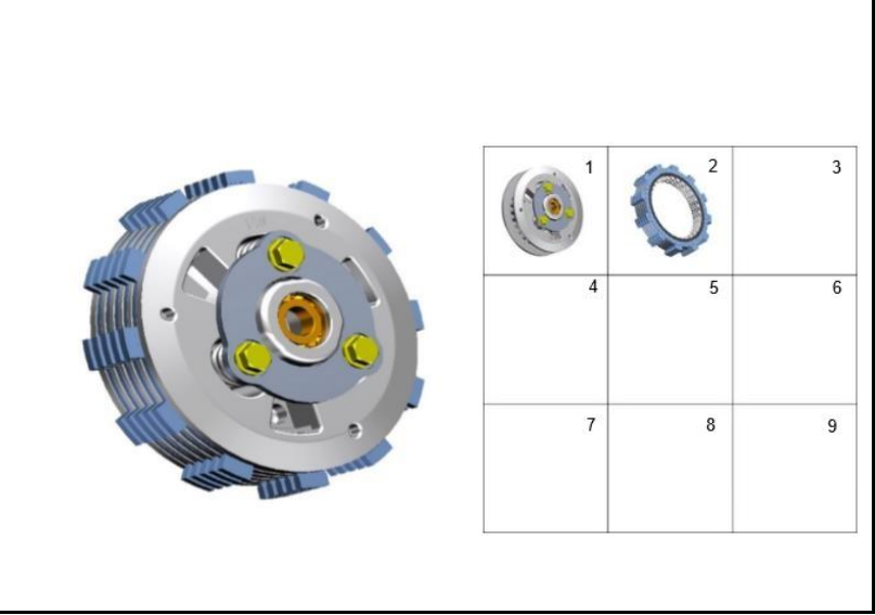
FIGURA 125: CLUTCH 2
