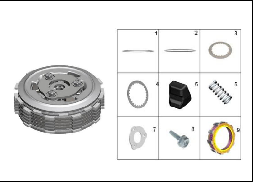
FIGURA 103: CLUTCH 3
