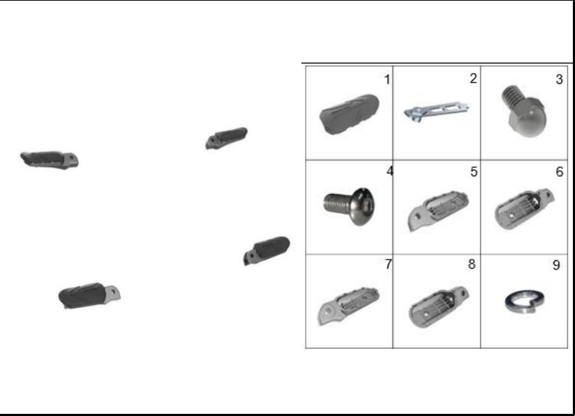
FIGURA 85: BASE REPOSAPIE
