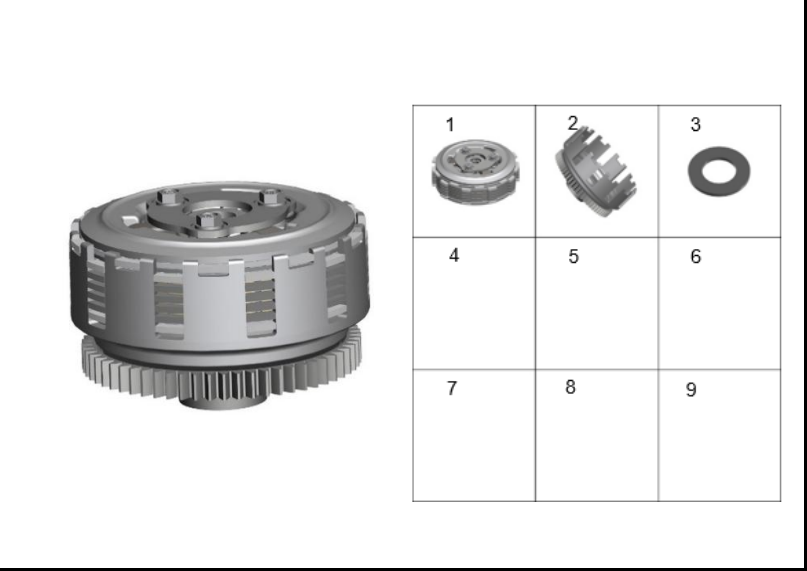
FIGURA 102: CLUTCH 2
