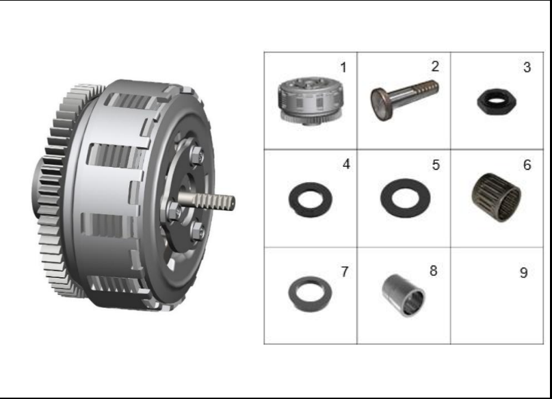
FIGURA 101: CLUTCH
