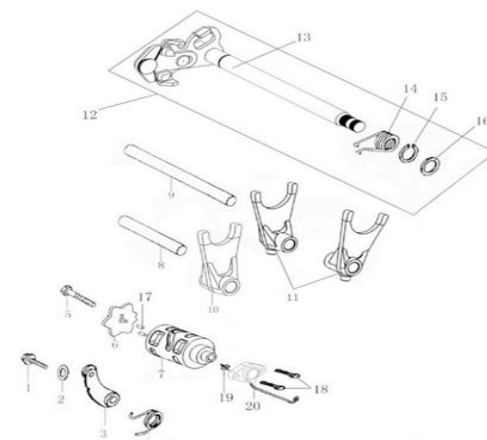
变速机构 GEARSHIFT MECHANISM
