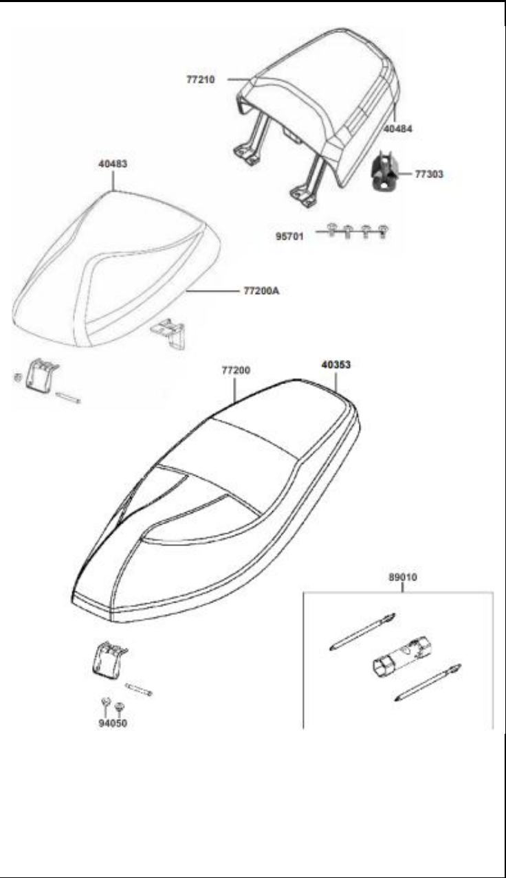
FIGURA 18: SILLÍN (1/2)
