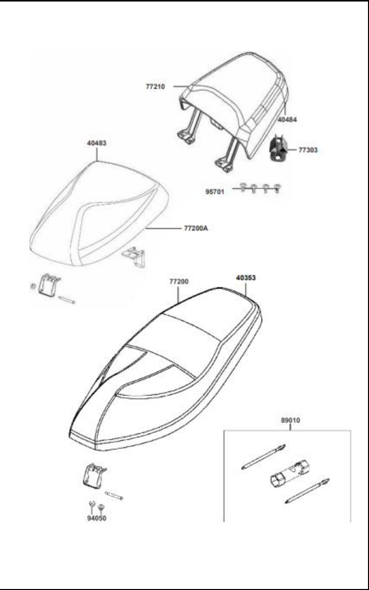
FIGURA 18: SILLÍN (2/2)
