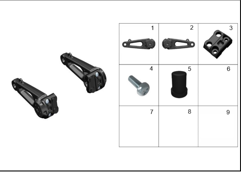
FIGURA 4: BALANCIN VISOR 2
