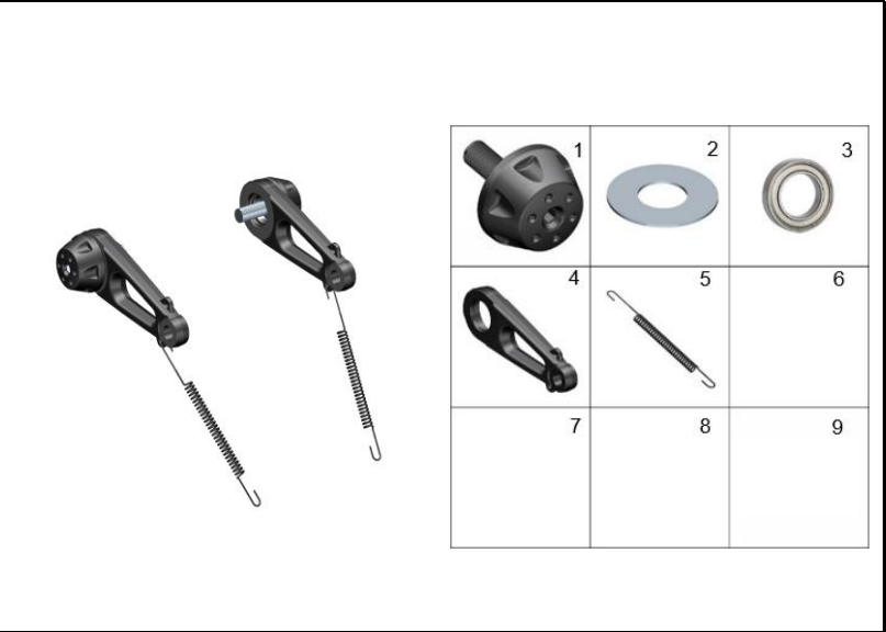
FIGURA 3: BALANCIN VISOR
