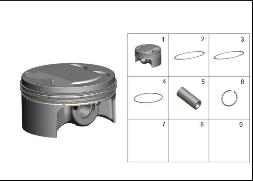
FIGURA 103: PISTON
