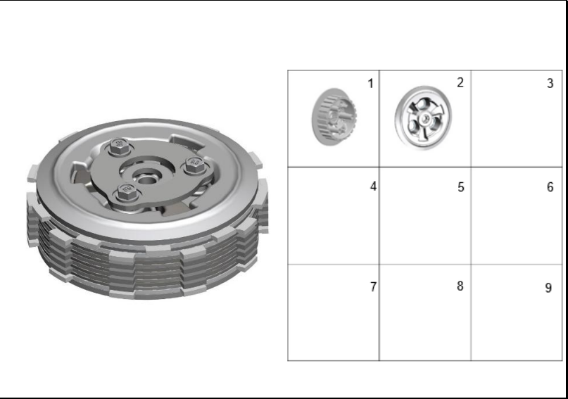
FIGURA 106: CLUTCH 4
