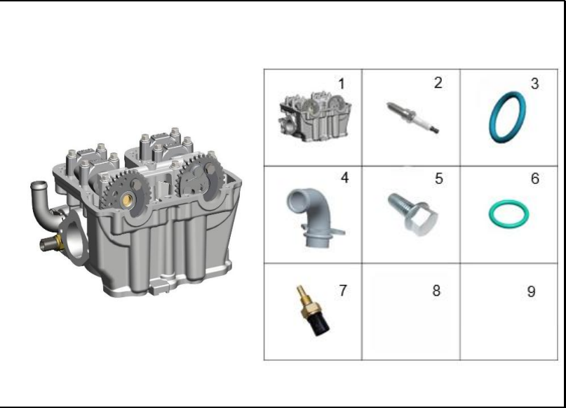
FIGURA 96: CULATA 2
