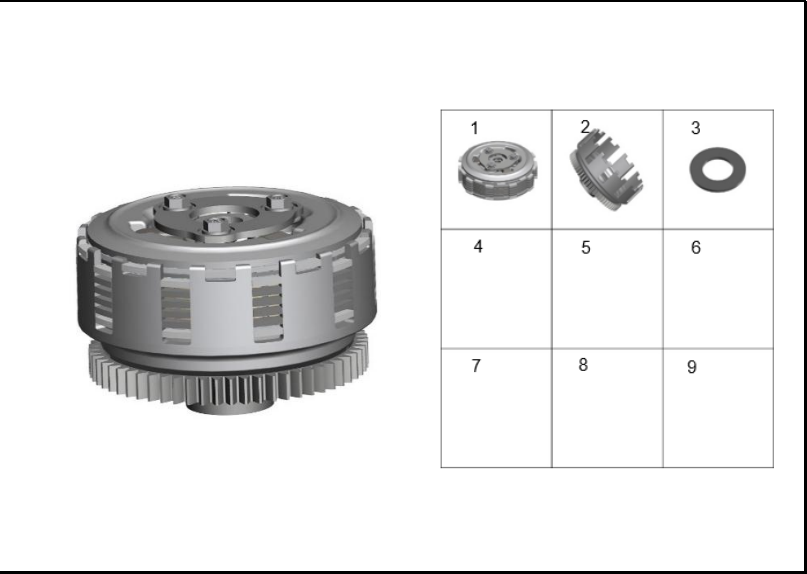
FIGURA 105: CLUTCH 2
