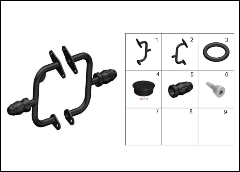
FIGURA 67: DEFENSAS
