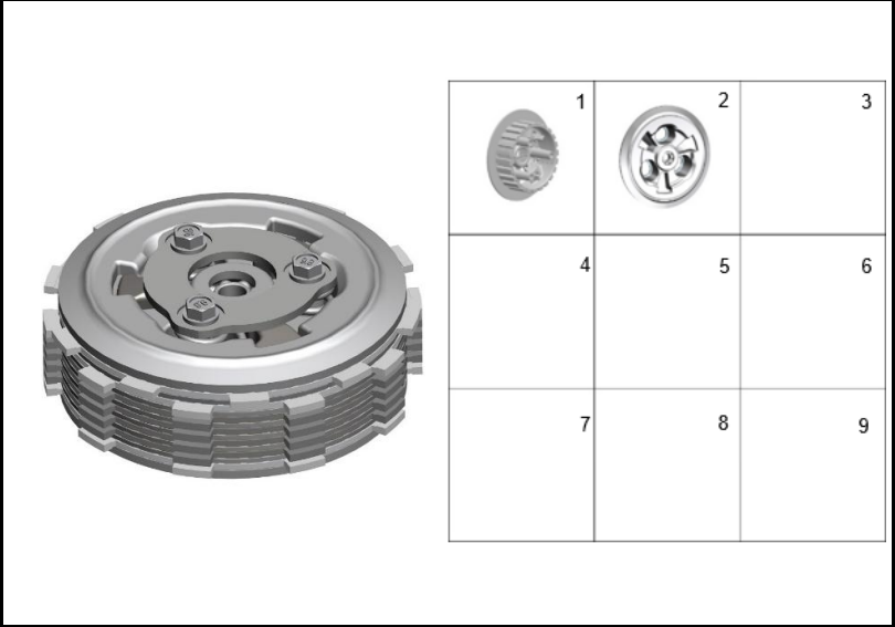
FIGURA 107: CLUTCH 4
