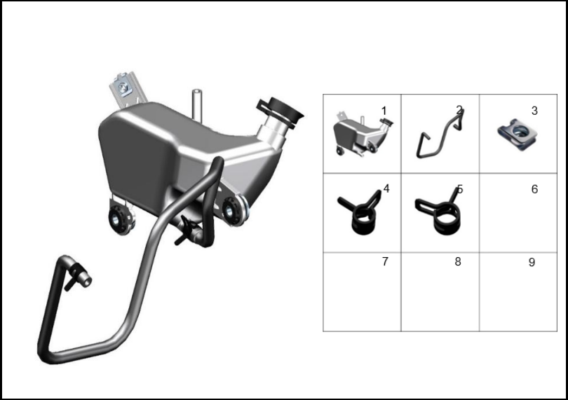
FIGURA 92: TANQUE RESERVORIO
