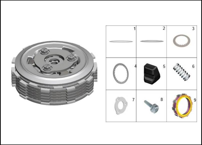
FIGURA 107: CLUTCH 3
