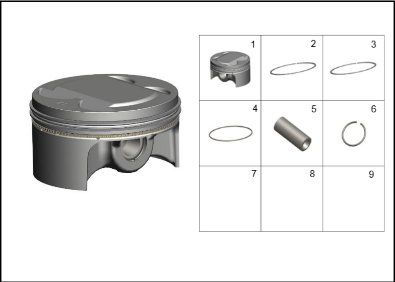
FIGURA 104: PISTON
