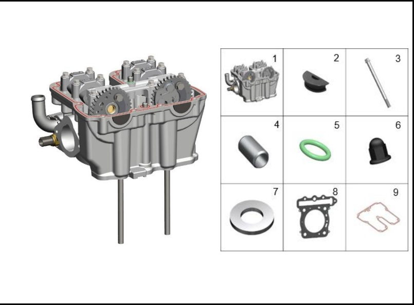
FIGURA 96: CULATA
