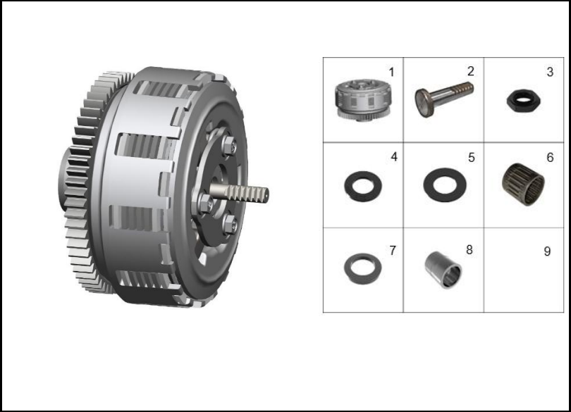
FIGURA 105: CLUTCH
