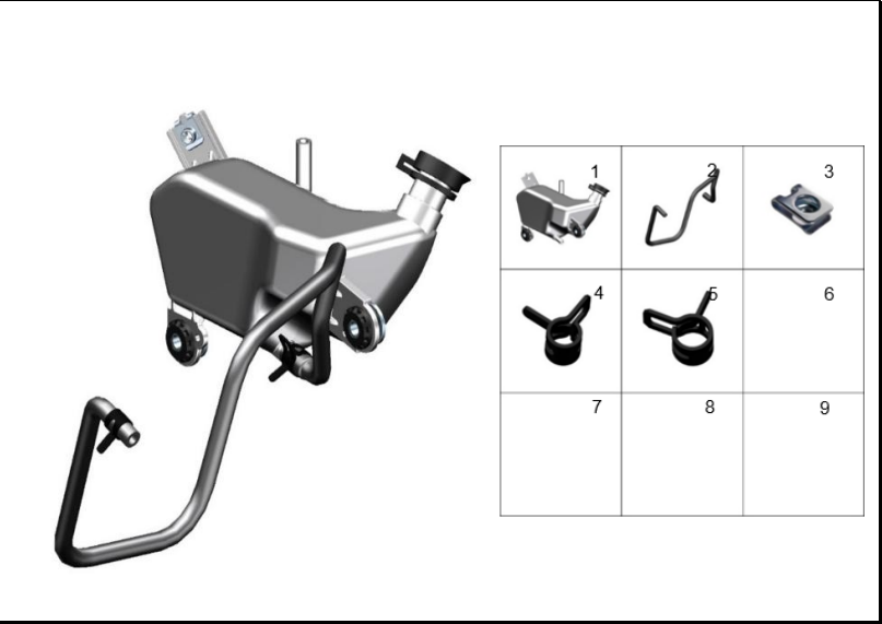
FIGURA 92: TANQUE RESERVORIO
