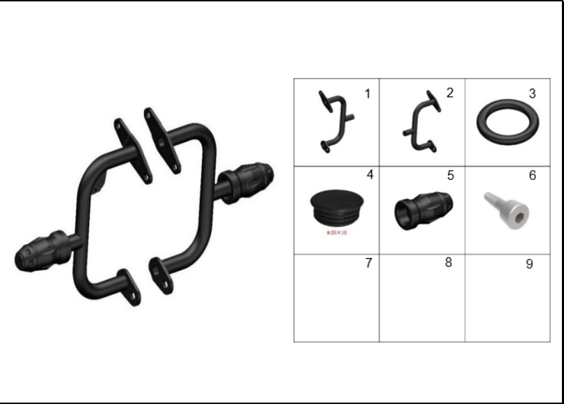
FIGURA 67: DEFENSAS
