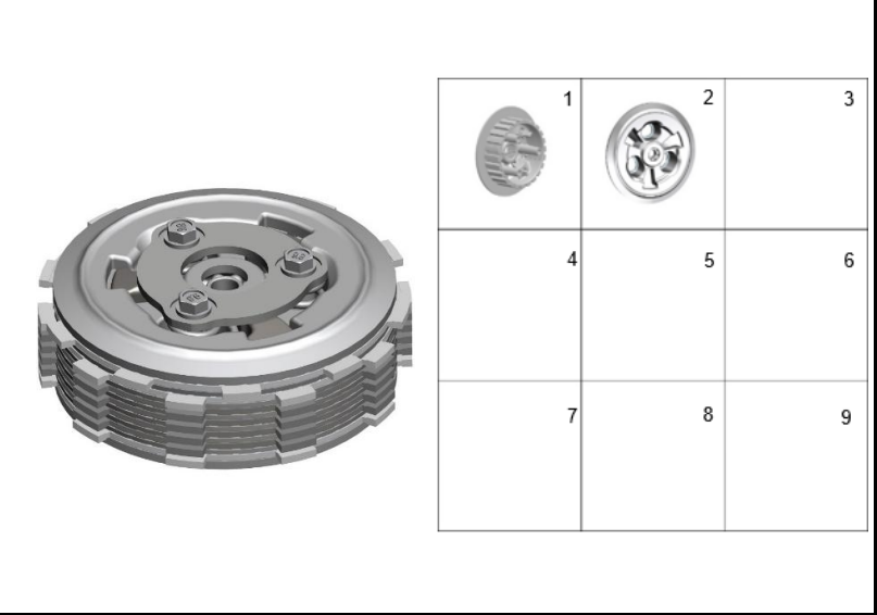
FIGURA 107: CLUTCH 4
