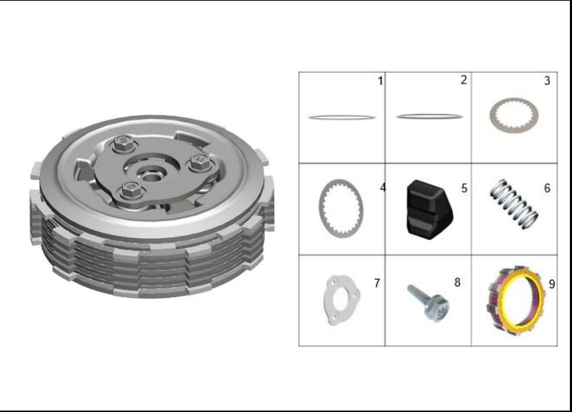
FIGURA 107: CLUTCH 3
