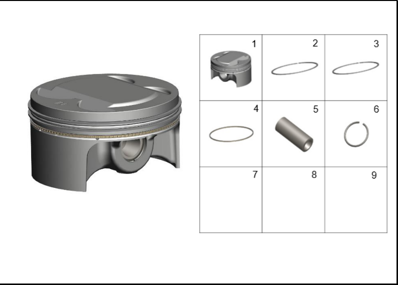
FIGURA 104: PISTON
