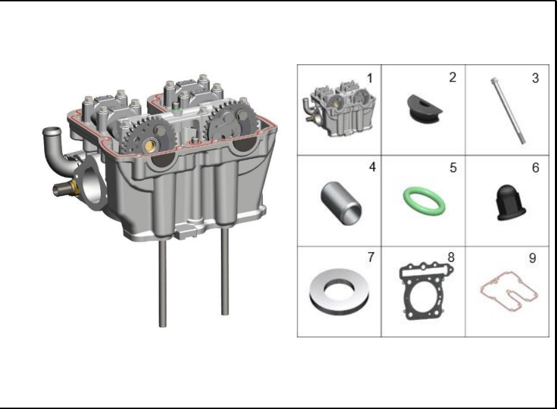
FIGURA 96: CULATA
