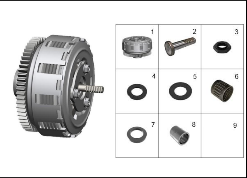
FIGURA 108: CLUTCH
