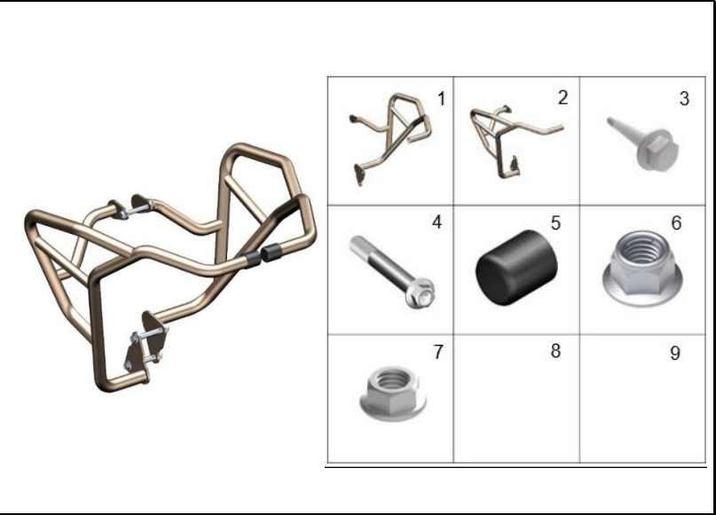
FIGURA 29: DEFENSAS
