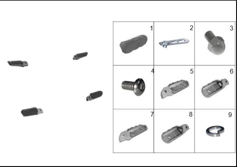
FIGURA 91: BASE REPOSAPIE
