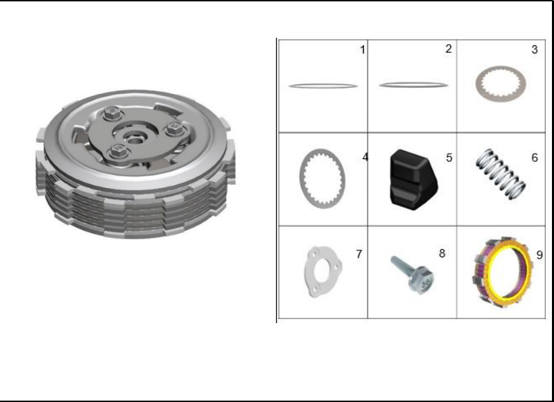
FIGURA 110: CLUTCH 3
