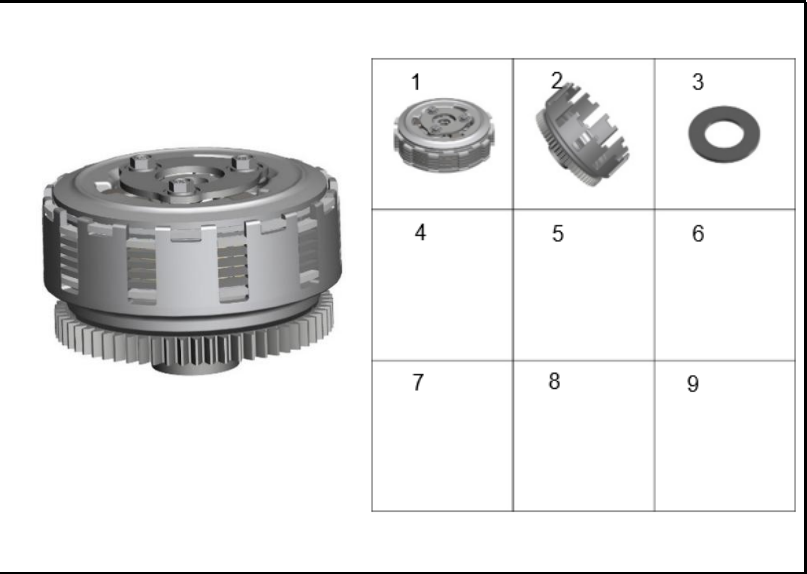
FIGURA 109: CLUTCH 2
