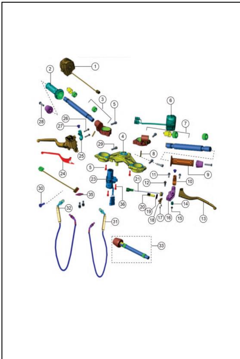
FIGURA N°20: MANUBRIO (2/2)
