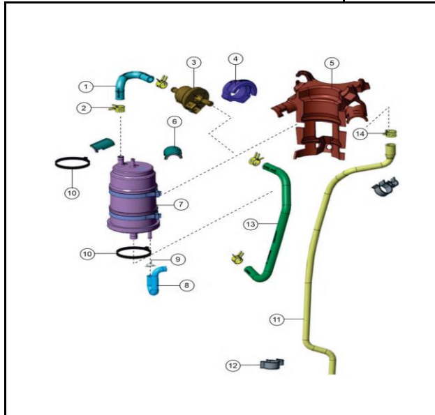
CANISTER
