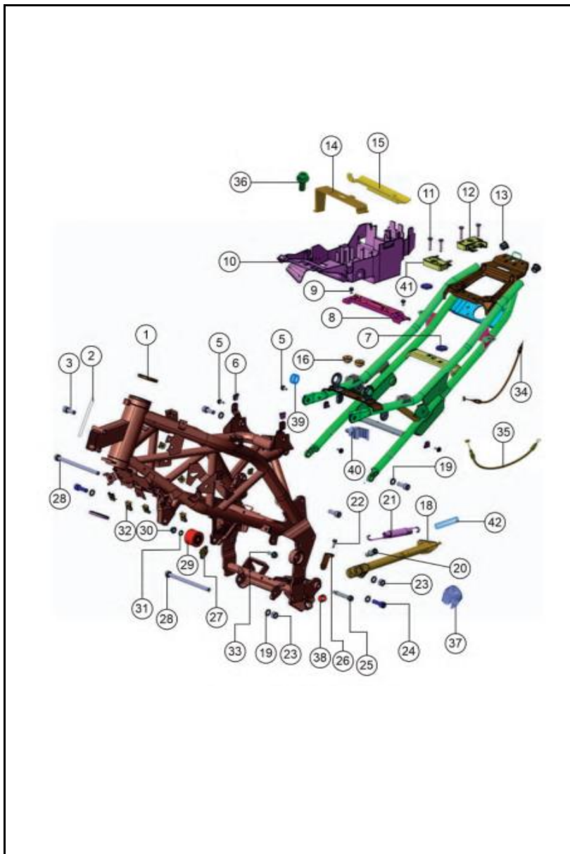
FIGURA N°21: CHASIS (2/2)
