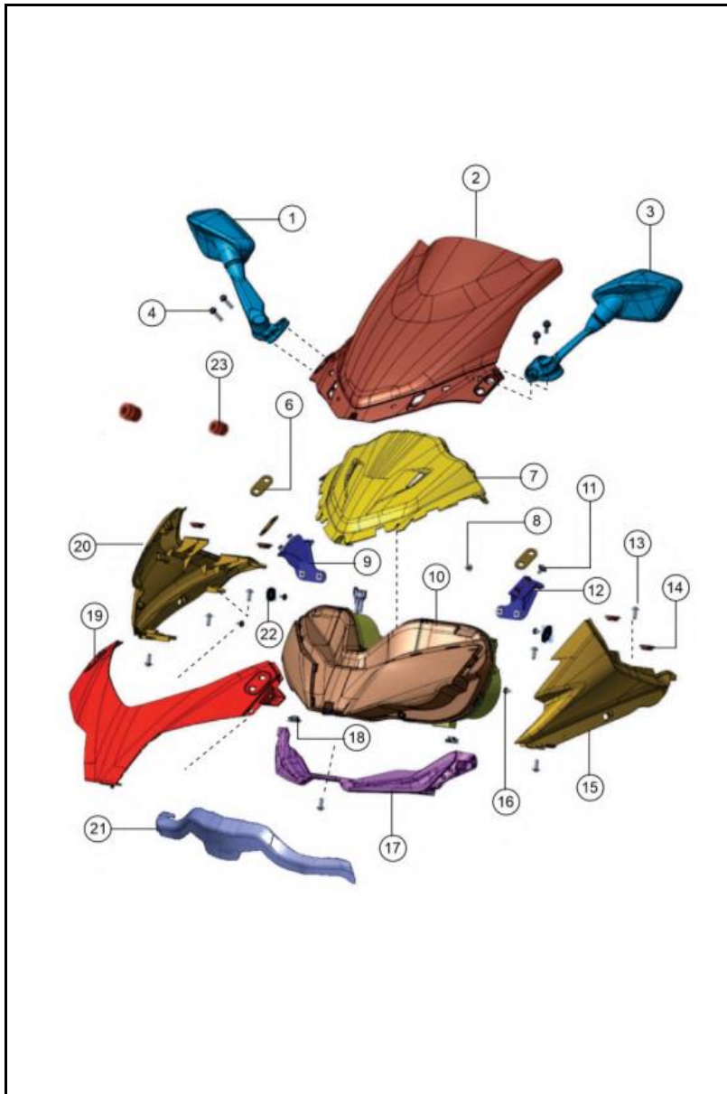
FIGURA N°17: FAROLA (1/2)
