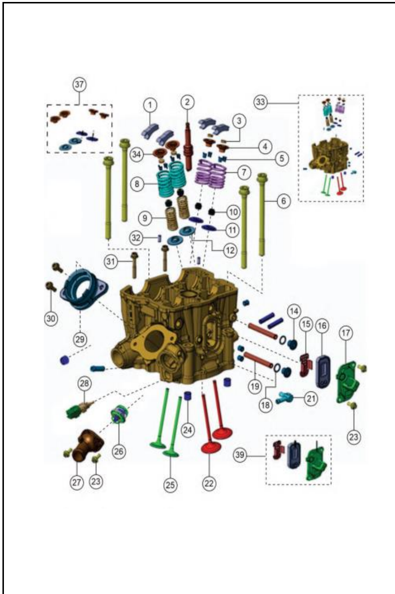
FIGURA N° 2: CULATA / VALVULAS (1/3)
