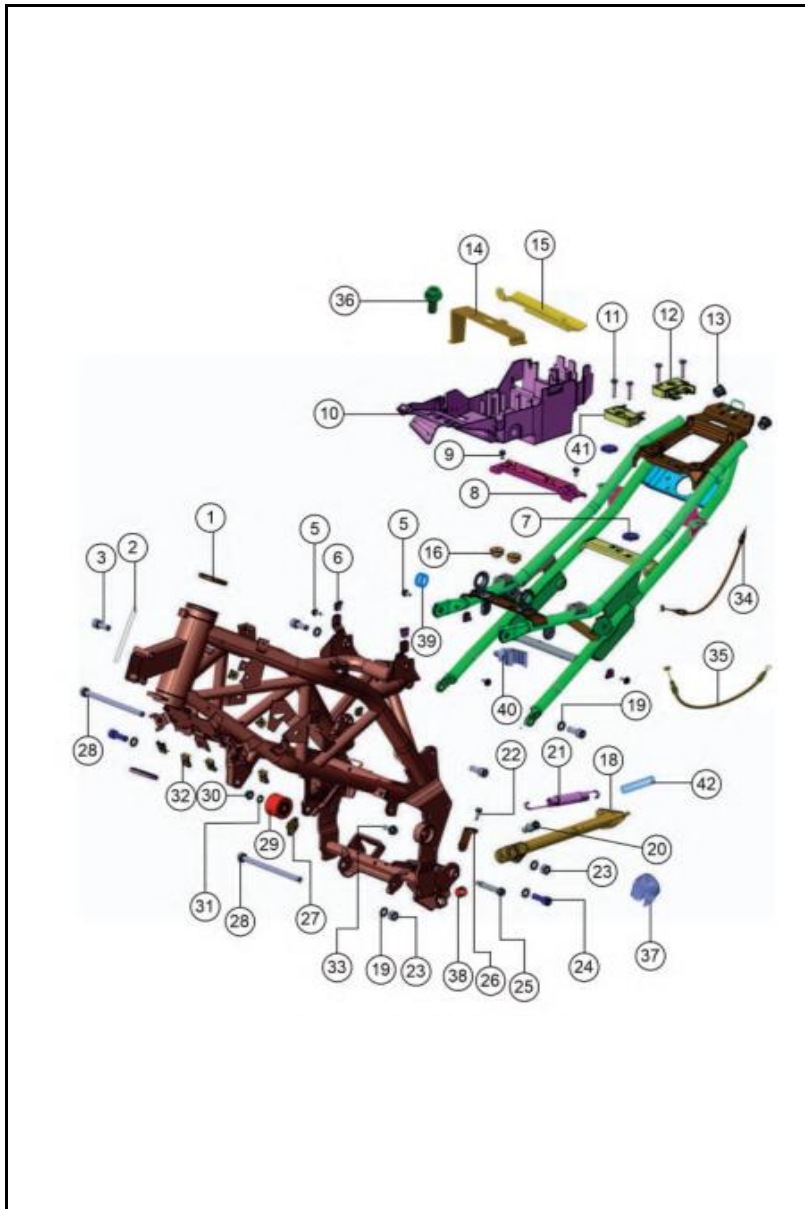
FIGURA N°21: CHASIS (1/2)
