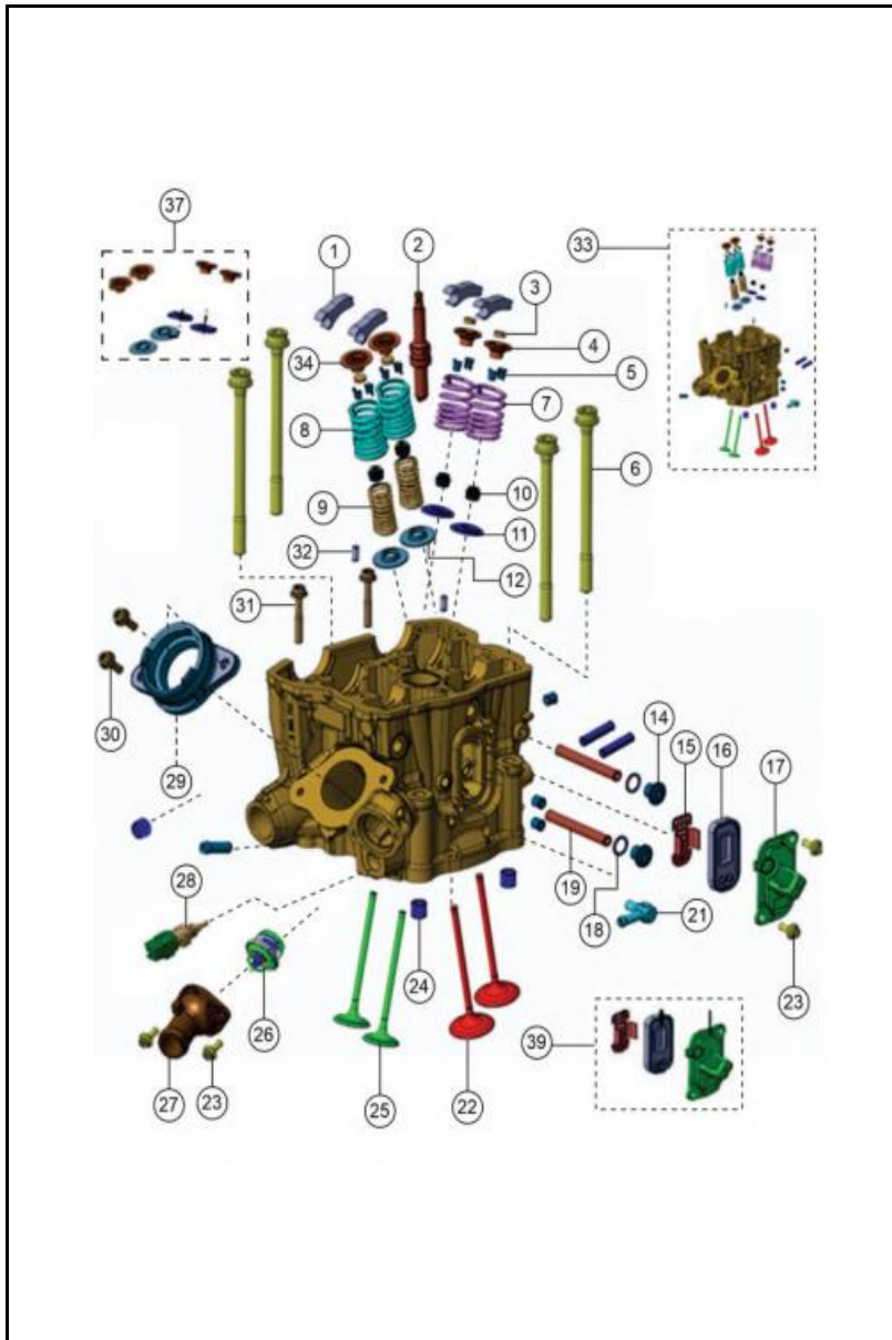
FIGURA N°2: CULATA / VALVULAS (2/3)
