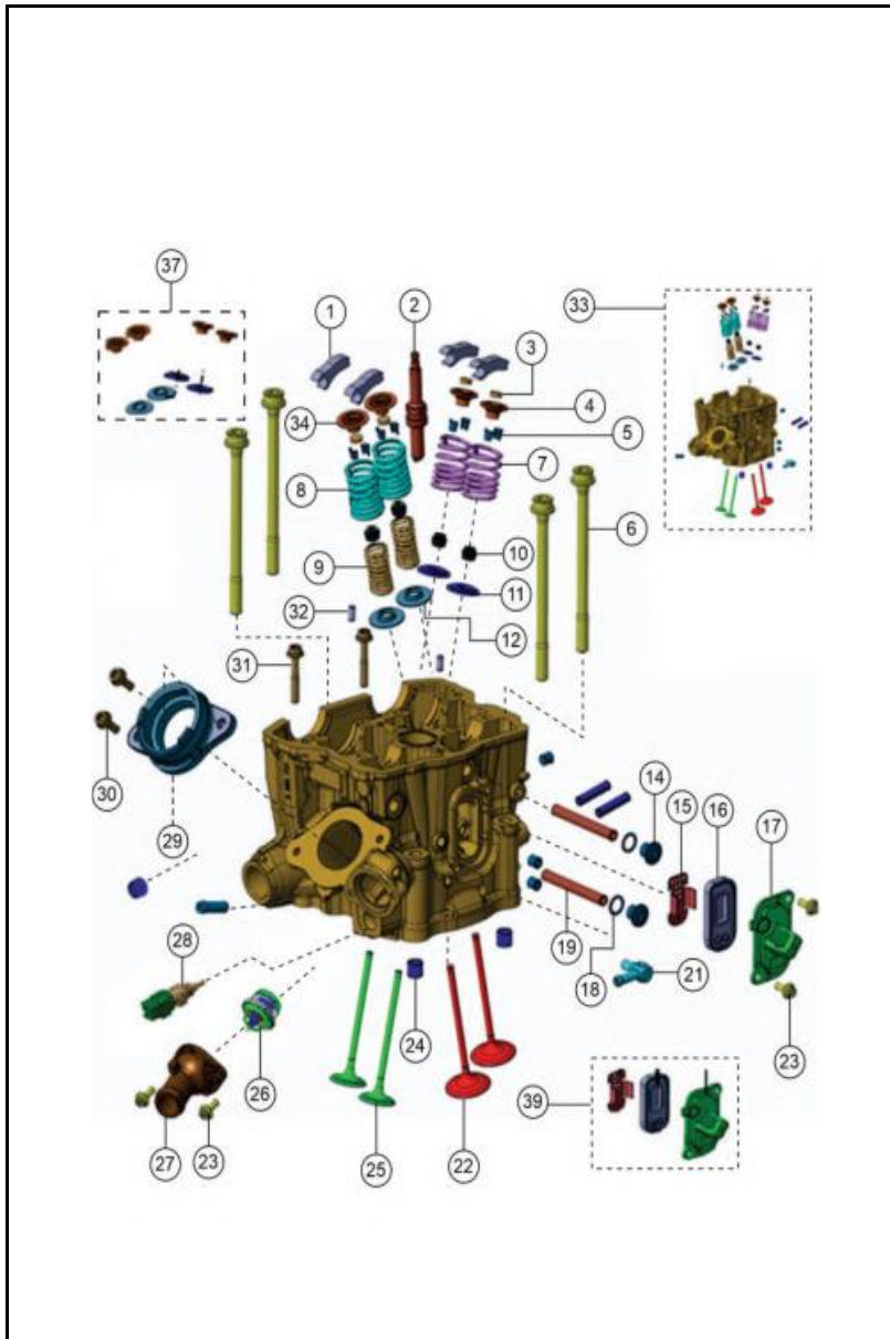
FIGURA N°2: CULATA / VALVULAS (3/3)
