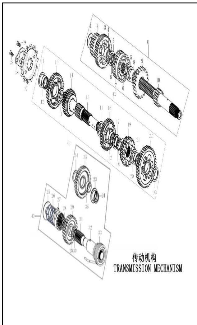
FIGURA N° 8: TRANSMISION (2/2)
