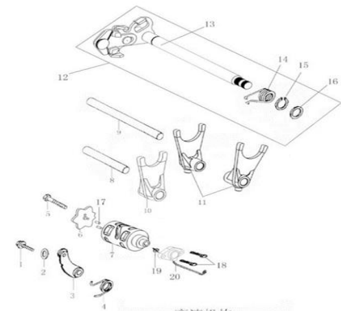
变速机构 GEARSHIFT MECHANISM
