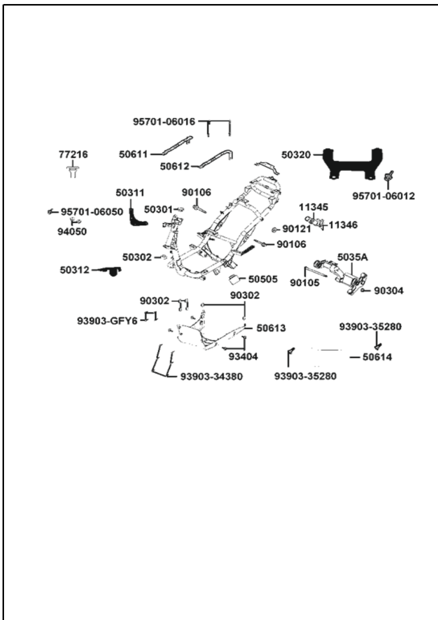
FIGURA N°29: CHASIS
