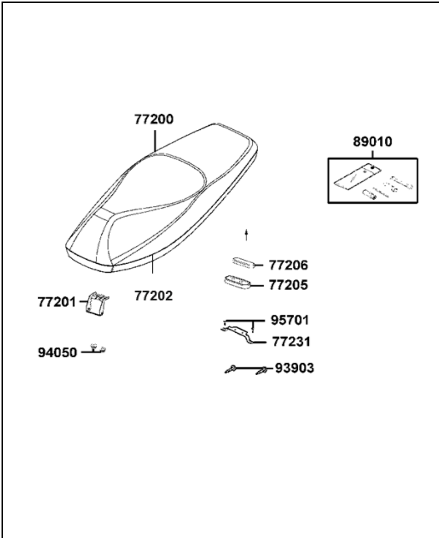
FIGURA N°18: SILLÍN
