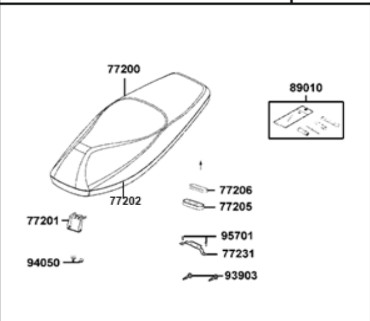
FIGURA 18: SILLÍN
