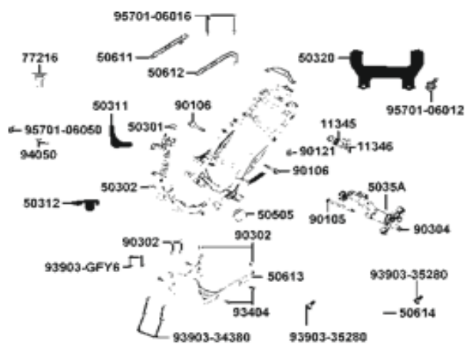
FIGURA 29: CHASIS
