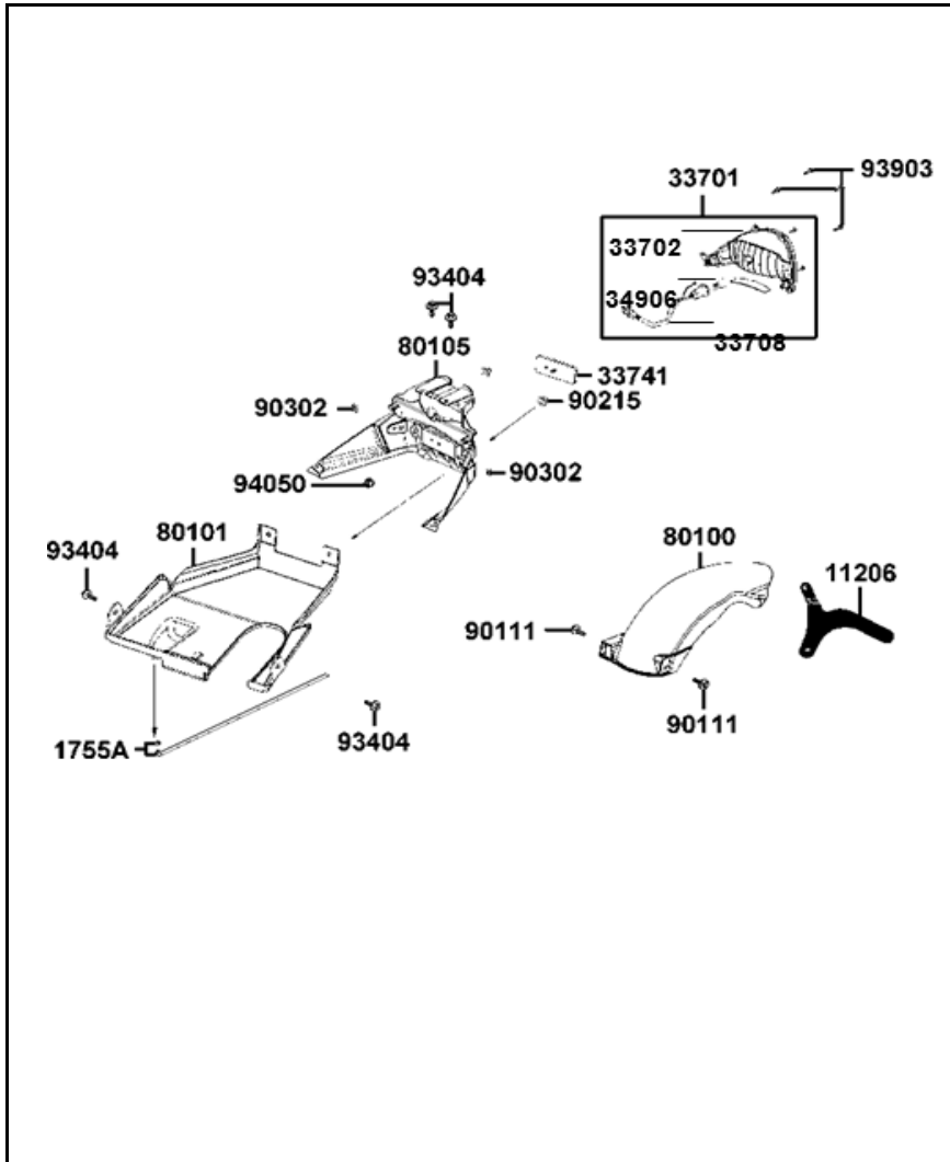
FIGURA N°27: STOP - GUARDABARRO TRASERO
