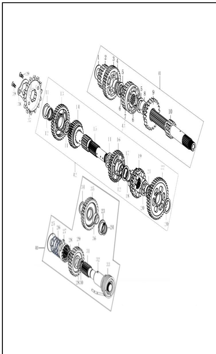
FIGURA N° 8: TRANSMISION (1/2)
