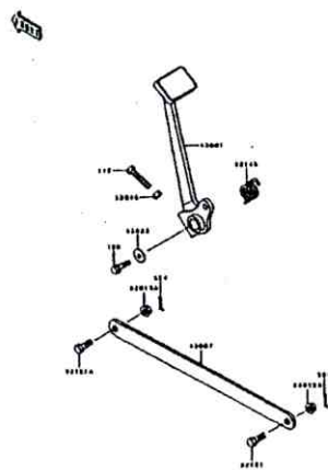
E-3 Brake Pedal
