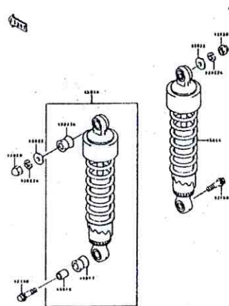
D-6 Suspension/Shock Absorber
