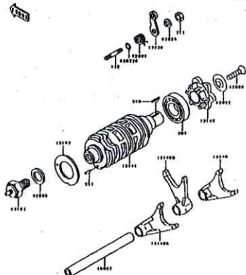
B-12 Gear Change Drum/Shift Fork(s)
