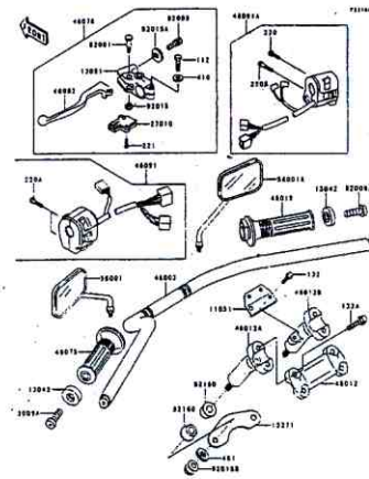
E-7 Handlebar(BN175-A3)
