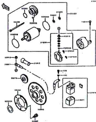
C-11 Starter Motor
