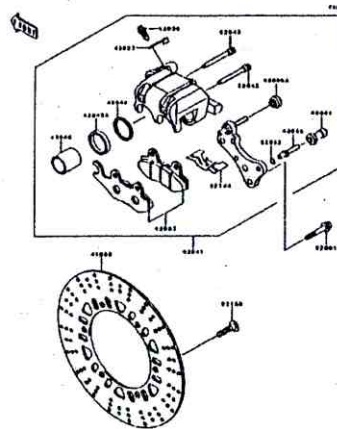
E-5 Front Brake
