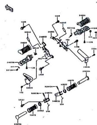
D-7 Footrests
