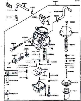
C-7 Carburetor(2/2)(BN175-A3)
