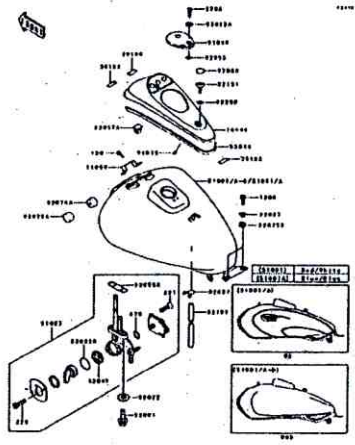
E-9 Fuel Tank
