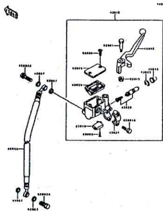
E-4 Front Master Cylinder
