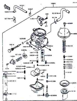
C-6 Carburetor(1/2)(BN175-A3)
