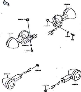
F-4 Turn Signals
