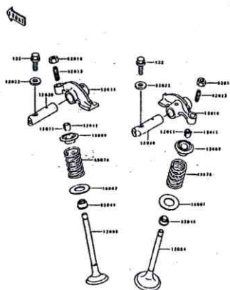
B-7 Valve(s)
