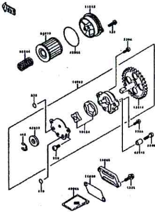
C-8 Oil Pump
