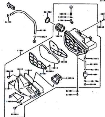
B-5 Air Cleaner
