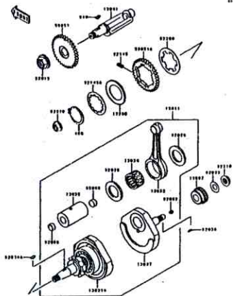
B-9 Crankshaft
