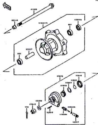
D-13 Front Hub
