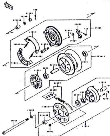
D-14 Rear Hub
