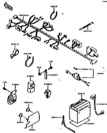
F-5 Chassis Electrical Equipment
