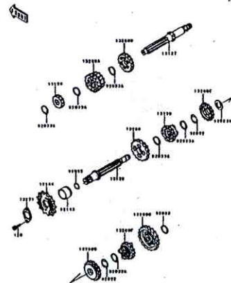
B-11 Transmission
