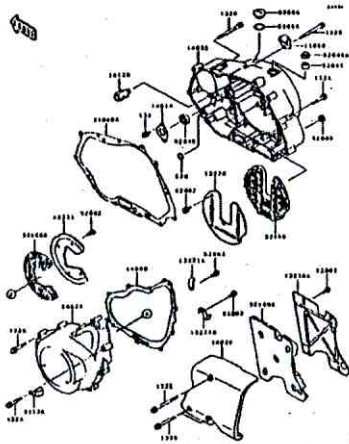
C-3 Engine Cover(s)
