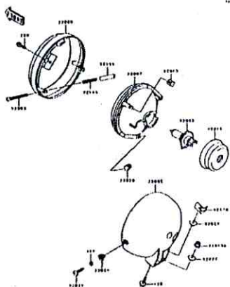
E-14 Headlight(s)
