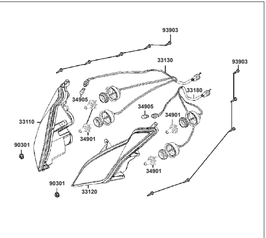
F01: FAROLA
