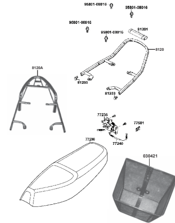
F-14: SILLÍN / AGARRADERA
