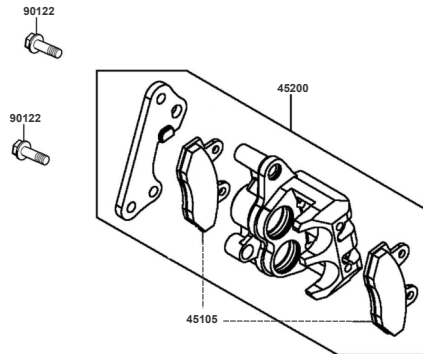
F-09: CALIPER
